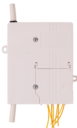
MTeH MINI – Riser Solution – Terminated on Pigtails
