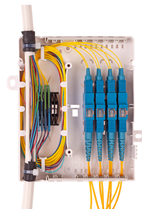
MTeH MINI – Riser Solution – Terminated on Pigtails
