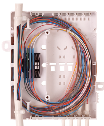
MTeH MINI – Riser Solution – Splicing Only
