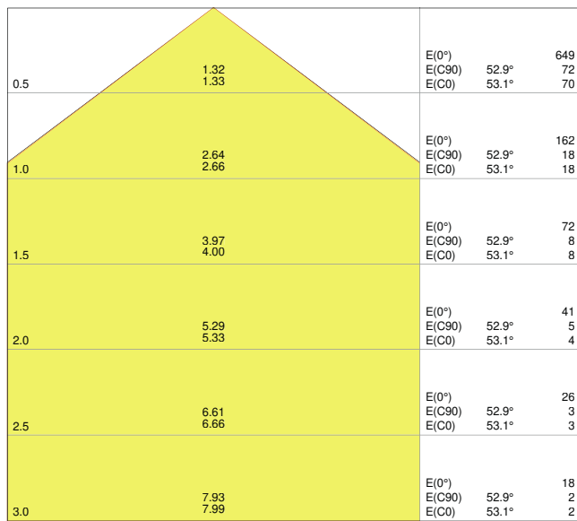
Distance [m] Cone diameter [m] Illuminance [lx] — C0/C180 (Half beam angle [°]: 106.2°) — C90/C270 (Half beam angle [°]: 105.8°)
