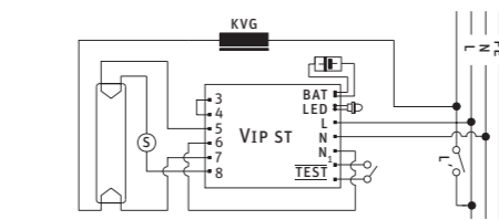
Fig.2. Supply-network and emergency mode with one fluorescent lamp (VIP ST)
