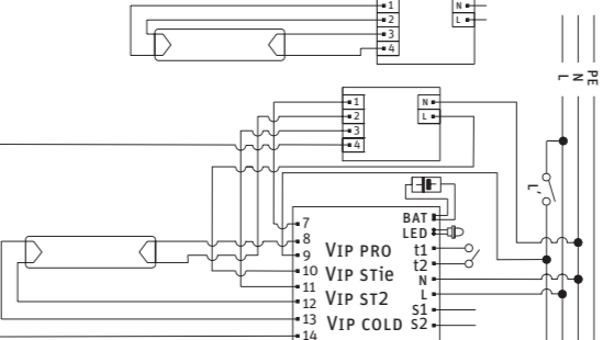
Fig.6. Supply-network and emergency mode with one fluorescent lamp in electronic ballast circuit (VIP PRO/VIP STie/VIP ST2/VIP COLD)
