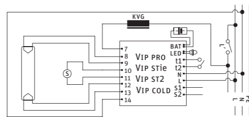
Fig.3. Supply network and emergency mode with one fluorescent lamp (VIP PRO/VIP STie/VIP ST2/VIP COLD)
