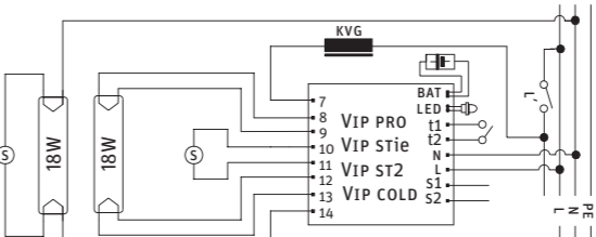
Fig.5. Supply-network and post current-decay mode with two fluorescent lamps 18 W (VIP PRO/VIP STie/VIP ST2/VIP COLD). Emergency mode with one fluorescent lamp.
