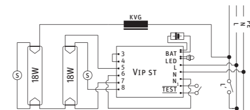
Fig.4. Supply-network and emergency mode with two fluorescent lamps 18 W (VIP ST) Emergency mode with one fluorescent lamp.
