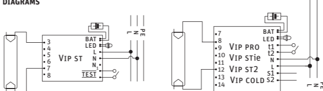
Fig. 1 Emergency mode with one fluorescent lamp (VIP ST, VIP PRO/VIP STie/VIP ST2/VIP COLD)
