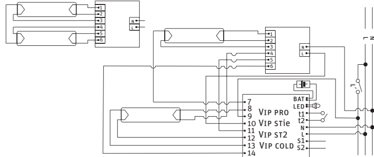
Fig.7. Supply-network and post-current decay mode with two fluorescent lamp in electronic ballast circuit (VIP PRO/VIP STie/VIP ST2/VIP COLD). Emergency mode with one fluorescent lamp.
