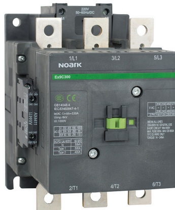
Frame size 300 Rated currents 225, 265, 300 A
