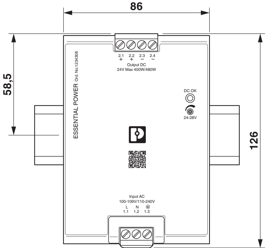
Dimensional drawing
