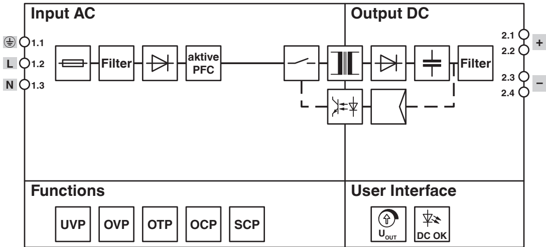
Block diagram
