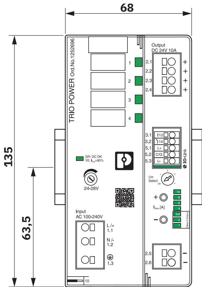
Dimensional drawing
