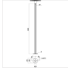
315024 Pole Spillo F.T. 2.8 m with flange Anthracite gray
