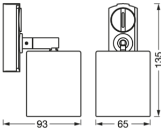
PGTRACKLIGHT SPOT MINICYLINDER WTGU10MiPRCmnk
