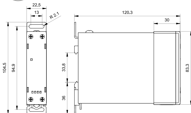
Type 77.x1 Screw terminal (plate clamp)
