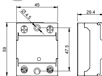
Type 77.x3 Screw terminal (plate clamp)
