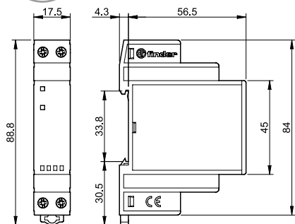
Type 77.x2 Screw terminal (plate clamp)
