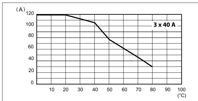
L77-23 Output RMS current v ambient temperature 77.B3.x.xxx.8671
