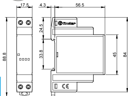
Type 77.01 DC Box clamp
