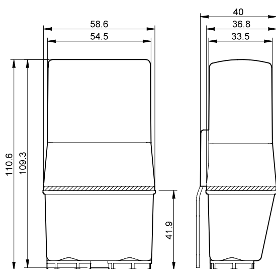
GPS external antenna , this device synchronizes the 12.B2s, 12.C1 time and date via Bluetooth. GPS excluded for countries: Russia and Iran.
