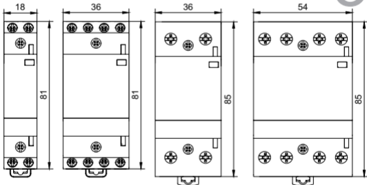
Ex9CH16/20/25H/32H
