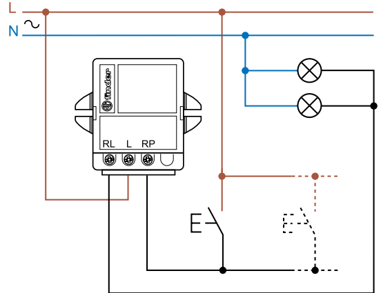
Type 15.91 - 4 wire connection
