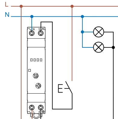
Type 15.81 - 4 wire connection
