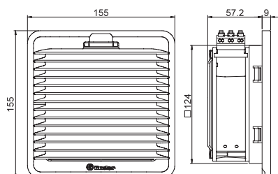
Type 7F.xx.x.xxx.2055 Push-in terminal
