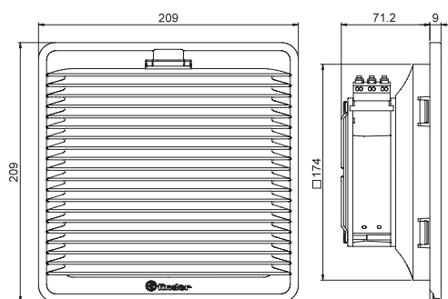
Type 7F.xx.x.xxx.3100 Push-in terminal
