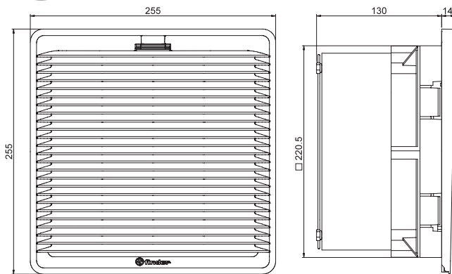
Type 7F.xx.x.xxx.4400 Push-in terminal
