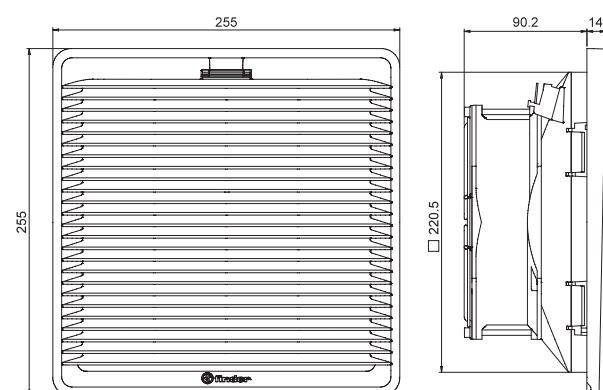
Type 7F.xx.x.xxx.4250 Push-in terminal
